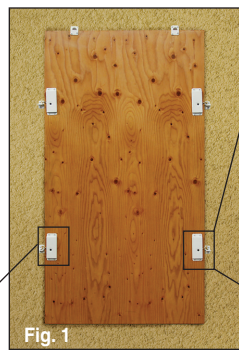
Fig. 1 A HURRICANE SHUTTER (A SHEET OF PLYWOOD) IS SURFACE MOUNTED WITH LEFT- AND RIGHT-HAND NORSE LATCHES AND BIG 'OT' RECEIVERS Fig. 2 THE TYPE 1R LATCH (RIGHT HAND SHOWN) CLAMPS THE PANEL FIRMLY AGAINST THE WINDOW FRAME. TYPE 1L (LEFT HAND) LATCH DOES THE SAME Fig. 3 HOOKS AND HANGERS ACCOMMODATE PANELS 1/4" TO 3/4" AND FIRMLY HOLD THE PANEL WHILE IT IS BEING INSTALLED, MAKING INSTALLATION VERY EASY. THE ANGLED HOOK/HANGER ENGAGEMENT ALSO FORCES THE PANEL INWARD AGAINST THE WINDOW FRAME. SEE TDSs 209-1A1 AND 209-1B1.
